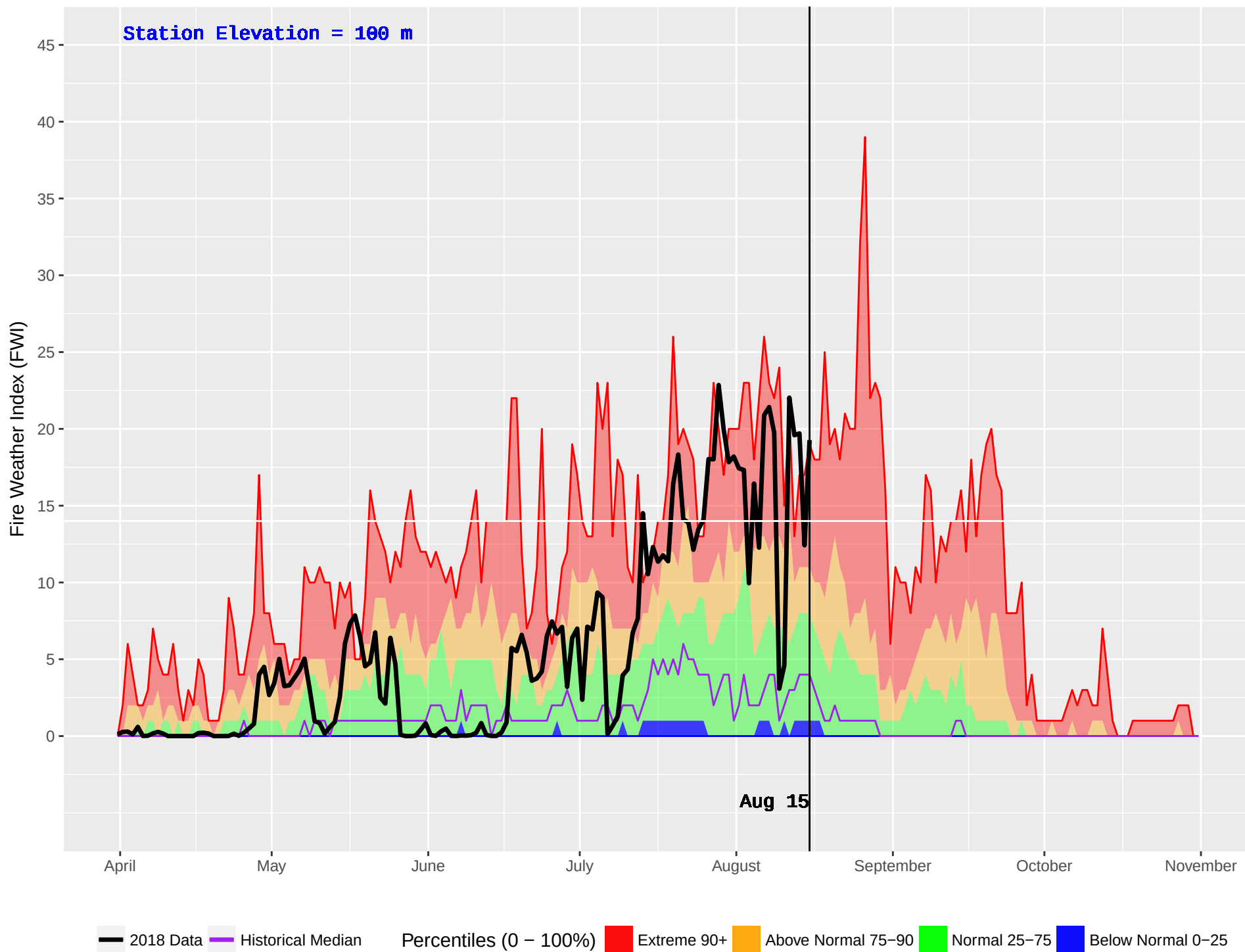
HONNA (93) : Historical (1986–2016) and Current (2018) Daily Fire Weather Index (FWI)
