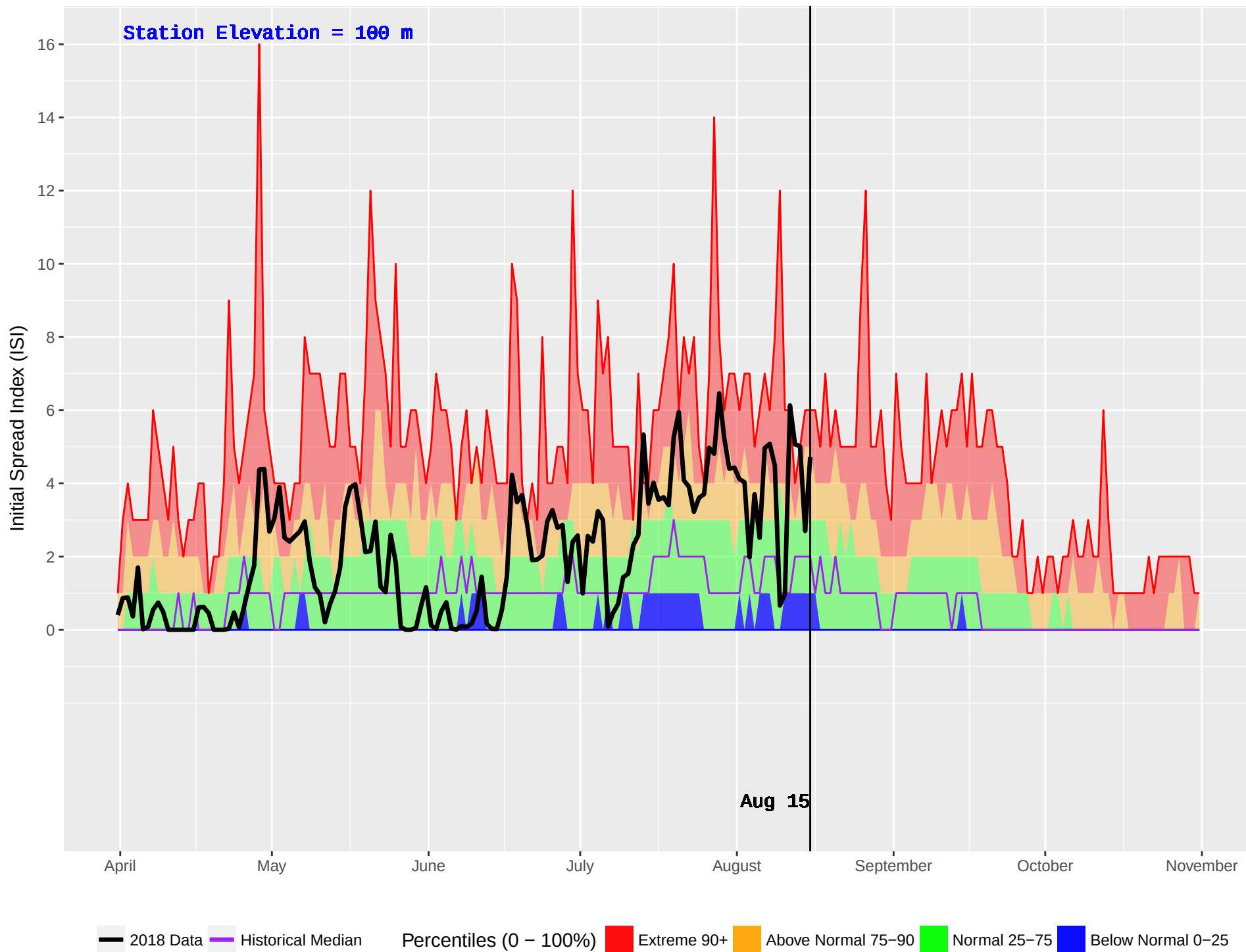
HONNA (93) : Historical (1986–2016) and Current (2018) Daily Initial Spread Index (ISI)
